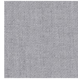
DN2-MTU-01 Beryllonite
